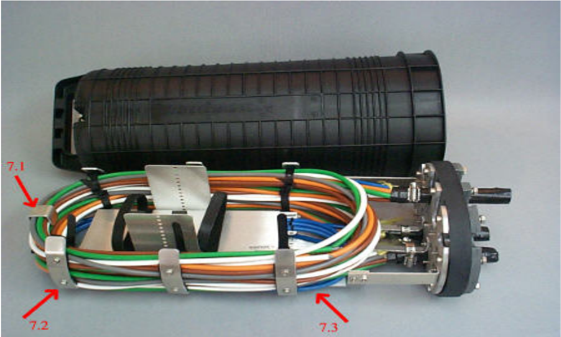
FIGURE 7 & 8: MID-SHEATH STORAGE BRACKETS FOR EXPRESS BUFFER TUBES 7.1, 8.1 express buffer tube storage 7.2, 8.2 mid-sheath storage bracket 7.3, 8.3 store spliced buffer tubes on bottom
